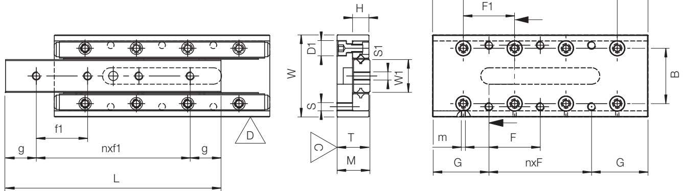
Abmessungen in mm · Dimensions in mm
