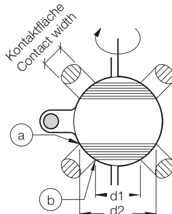
Detail B-B
