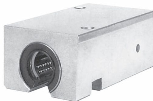
tandem open integrated wipers on both ends lubrication hole M8 x1
