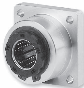
single flange integrated wipers on both ends
