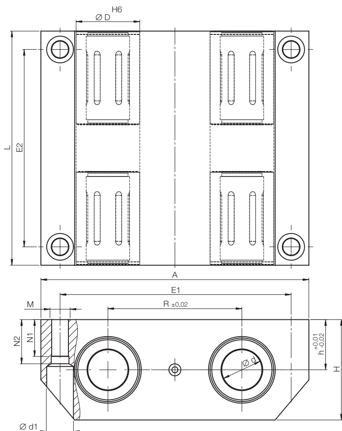
quadro closed compact version
