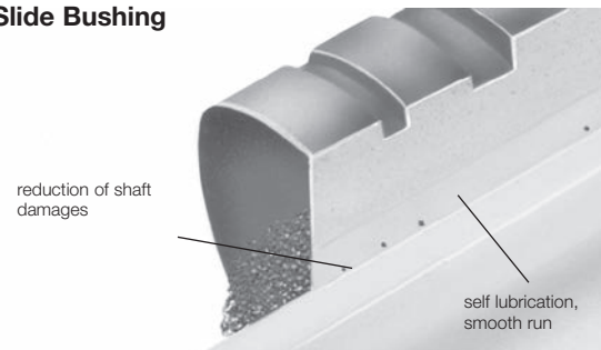
Slide Bushing
